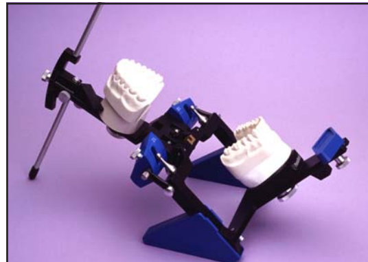
(6.) Open upper frame back to be supported by the support pin to facilitate laboratory procedures.
